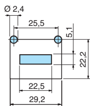
Rear fixing
