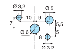
Rear fixing
