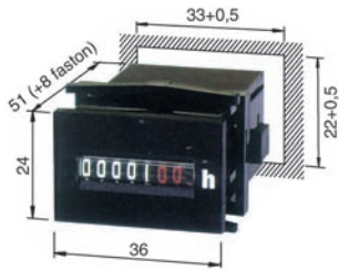
4RK30 Fast-on 6,3x0,8 mm with screws terminal
